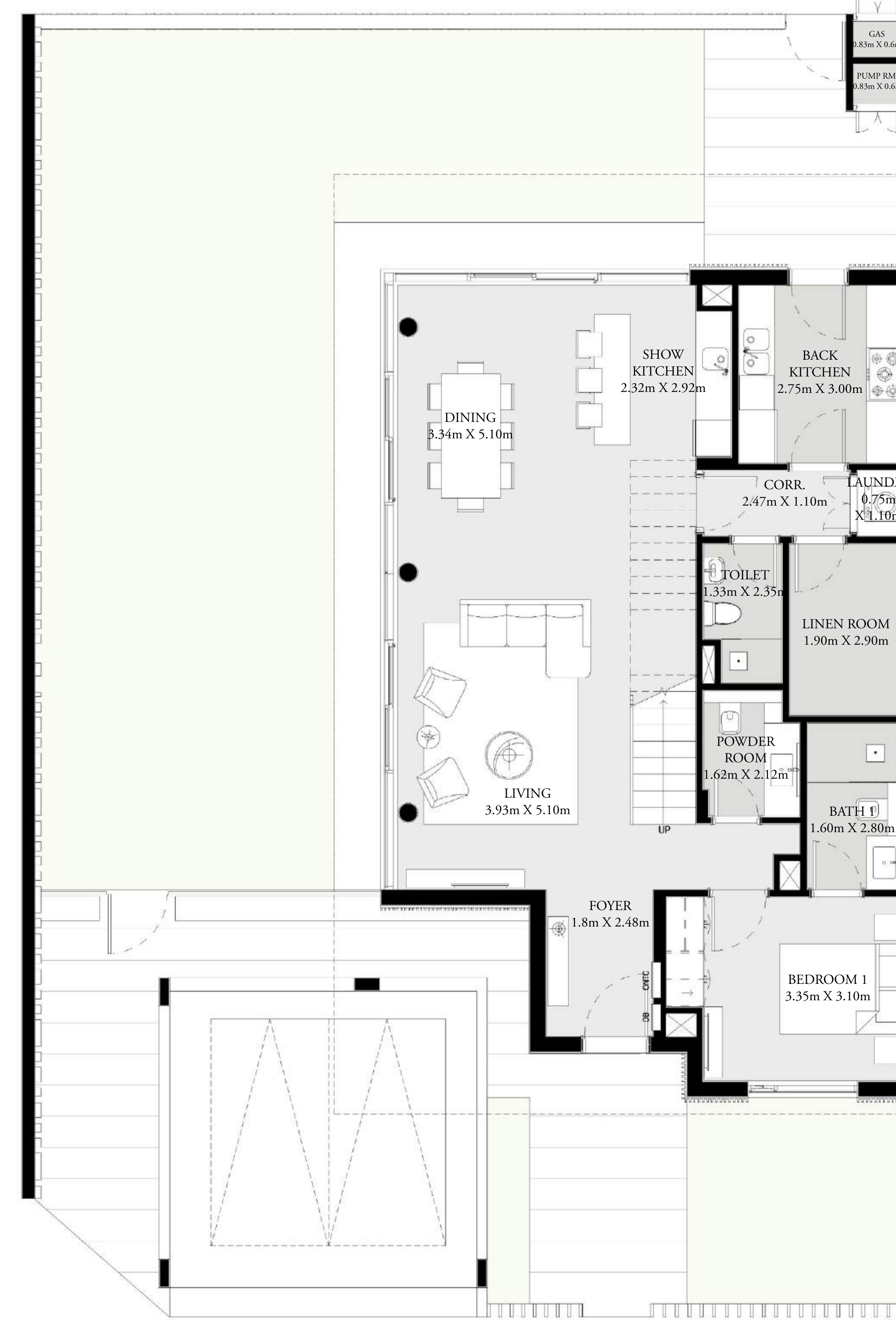
GROUND FLOOR
