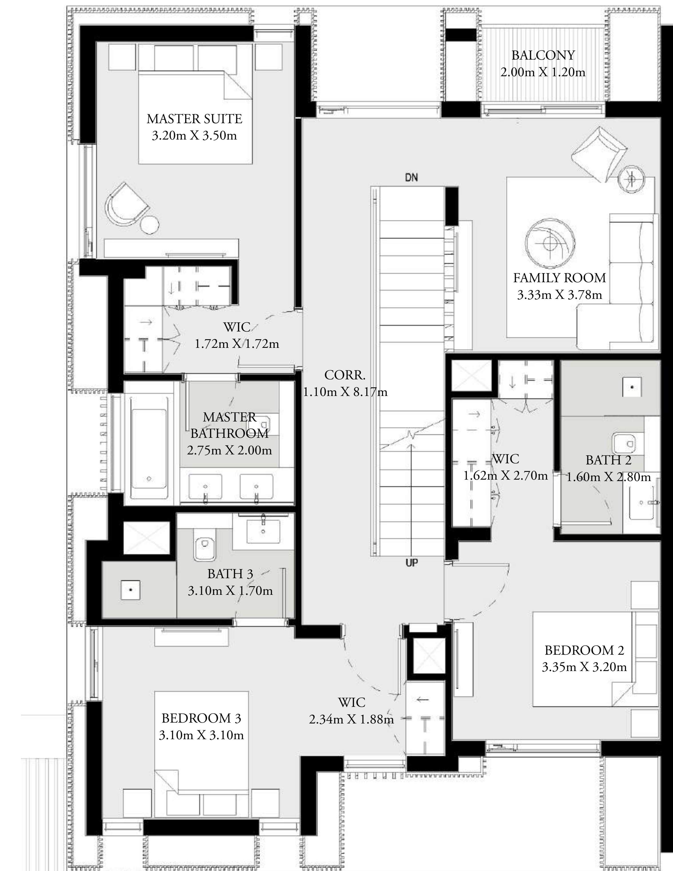
FIRST FLOOR
