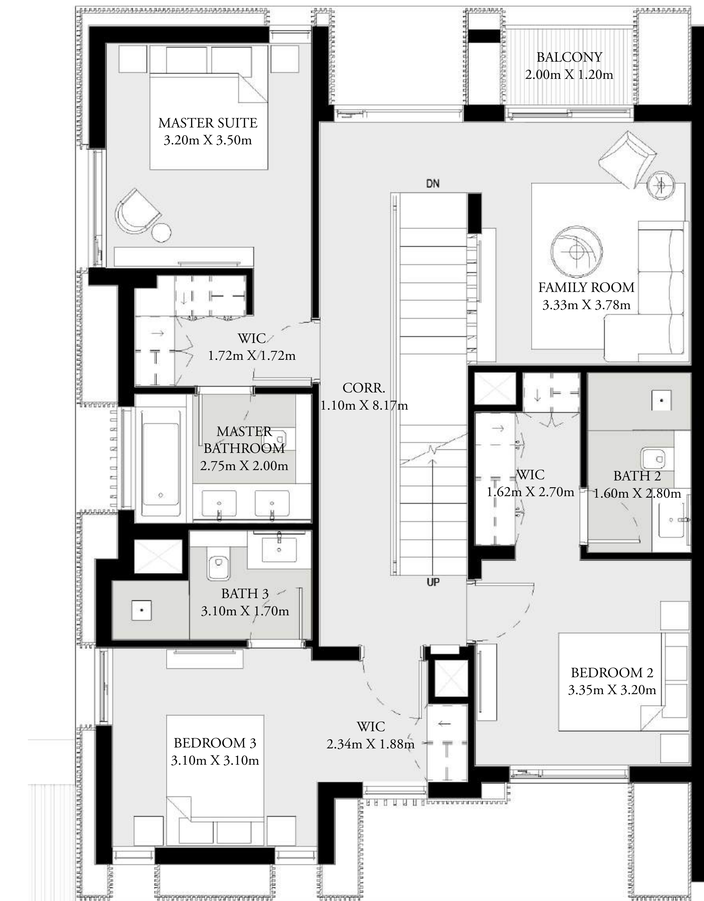
FIRST FLOOR
