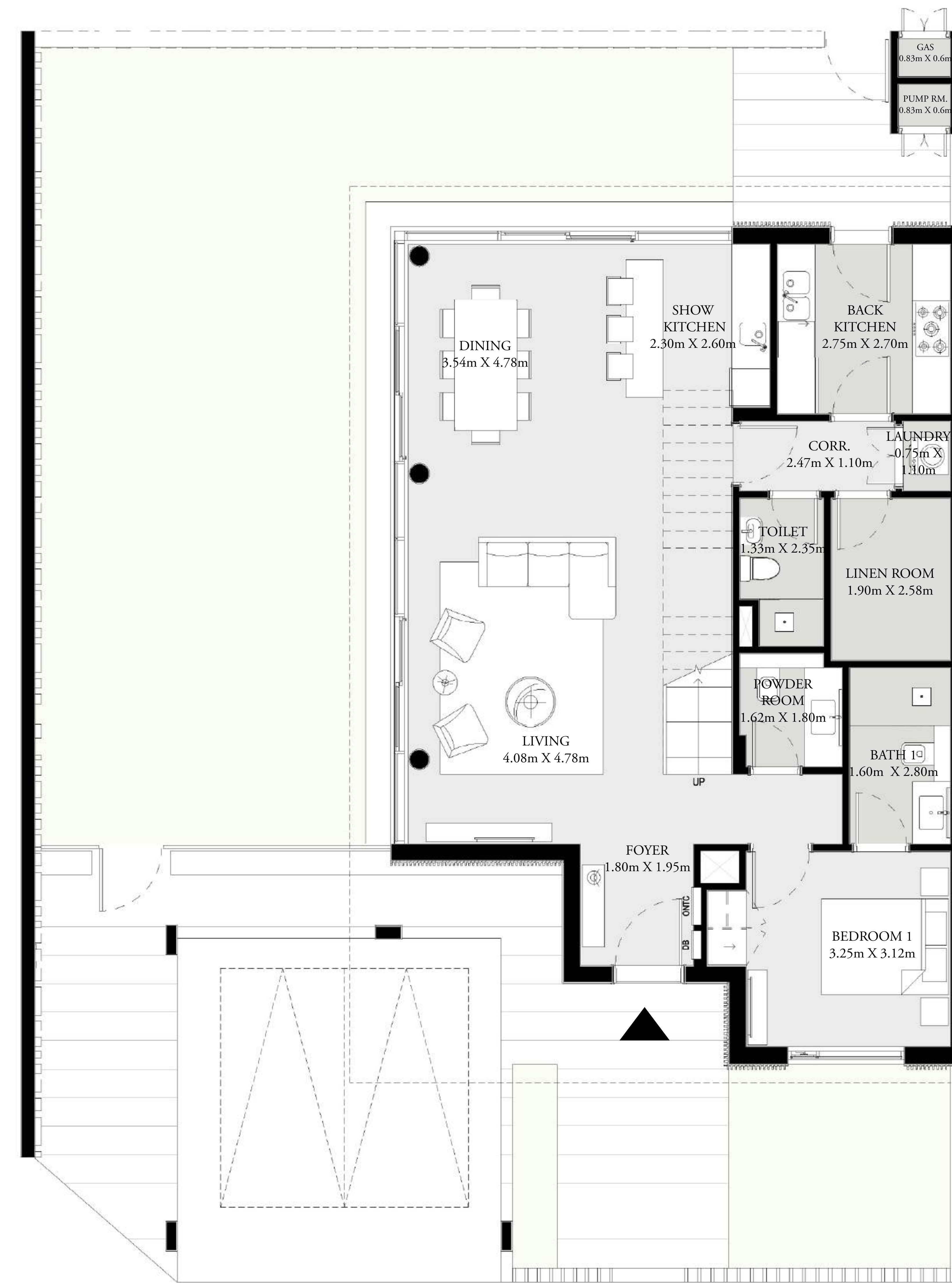
GROUND FLOOR
